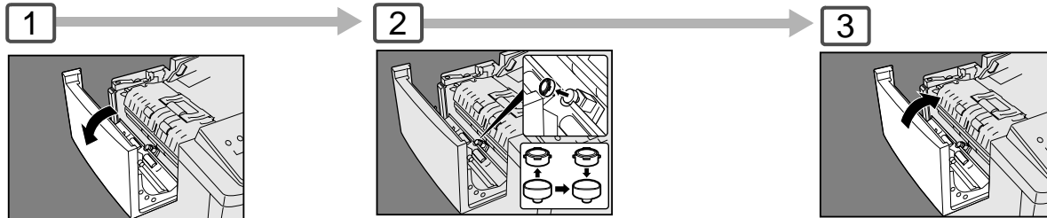
Open the ADF Cover
